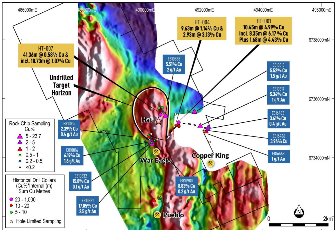
Figure 2: Summary map of existing work at the HAT prospect area over drone borne magnetic anomalism and including surface sampling and drilling highlights. Geophysics is 2024 1VD surveyed by Pioneer Exploration.
